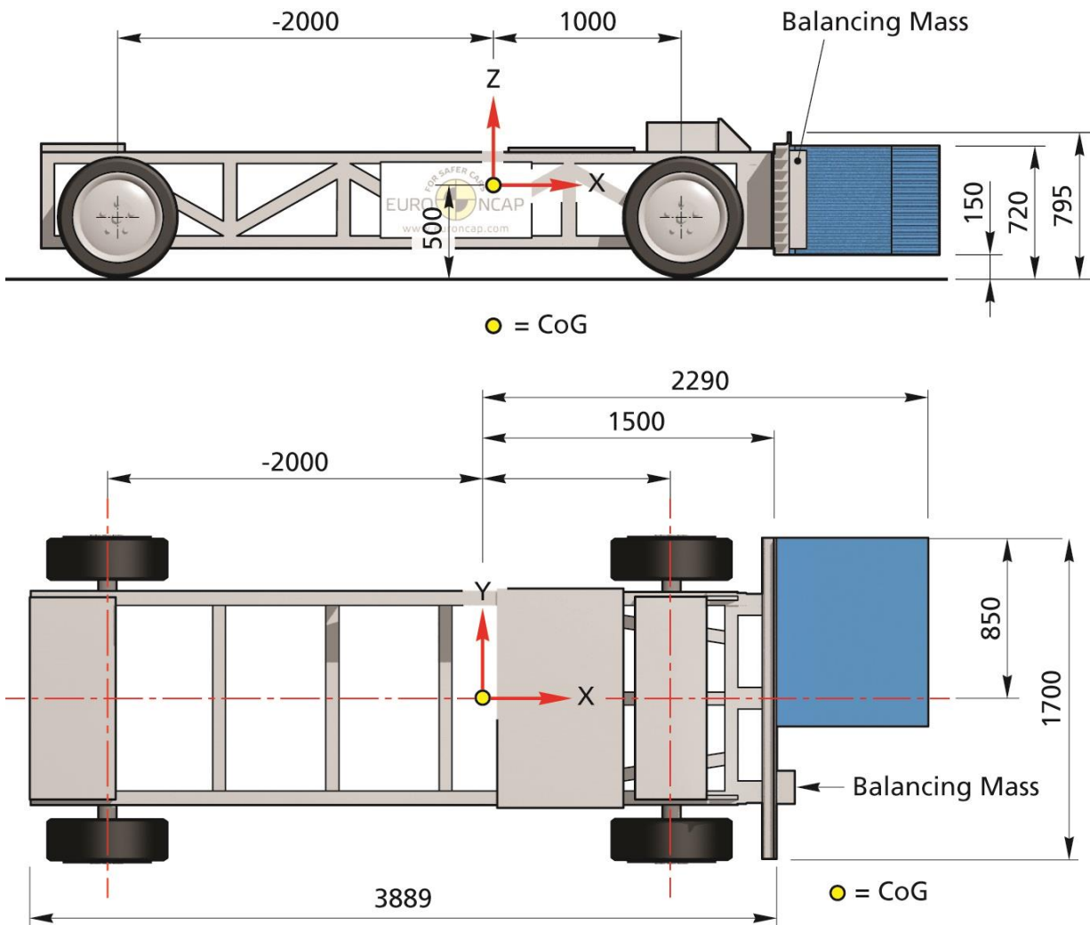
Figure 4 MPDB trolley
