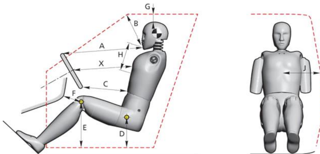
Figure 3 Dummy measurements
